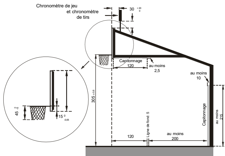
Figure 14 Module support de panier
